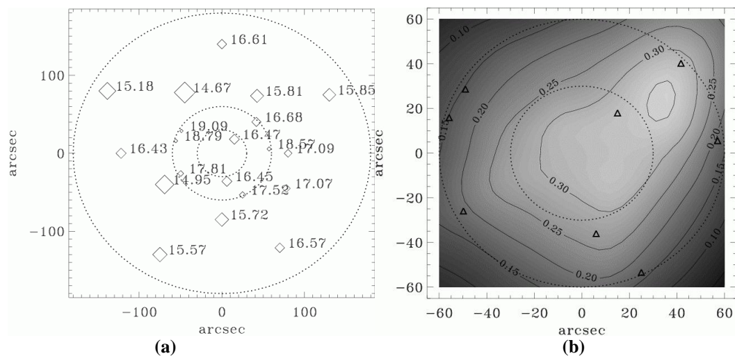
Figure 10. (a) Field map of the natural guide stars of the MfoV case with an inner 2' FoV and 6' FoV of the annular region, the two circles have diameters of 1' and 2'. The rumbles define the position of the stars and the numbers on the left are the magnitude in R band. (b) Strehl map of the same case, the NGS positions are indicated by the triangles.
