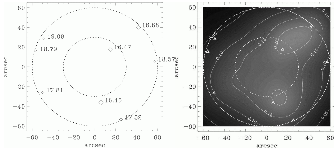
Figure 9. (a) Field map of the natural guide stars of the single FoV case with a single FoV of 2', the two circles have diameters of 1' and 2'. The rumbles define the position of the stars and the numbers on the left are the magnitude in R band. (b) Strehl map of the same case, the NGS positions are indicated by the triangles.
