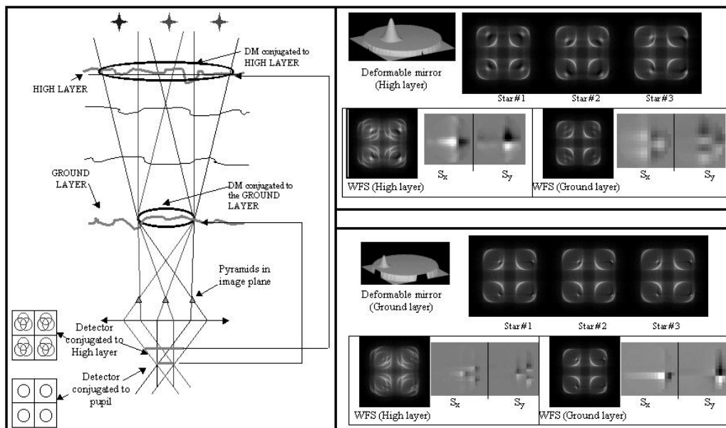
Figure 3. Left: LO concept . Right: Examples of simulated response of the WFSs when one actuator is driven in the deformable mirror conjugated to high layer (Top) and in ground layer (Bottom)
