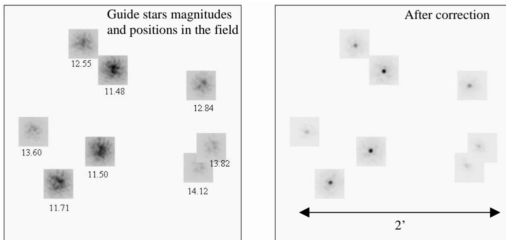
Figure 5. Simulation results of closed loop operation for an 8 stars asterism, long exposure of 1sec. The mean Strehl ratio in the Field is 38 % with a maximum strehl of 50 % for the brightest stars.
