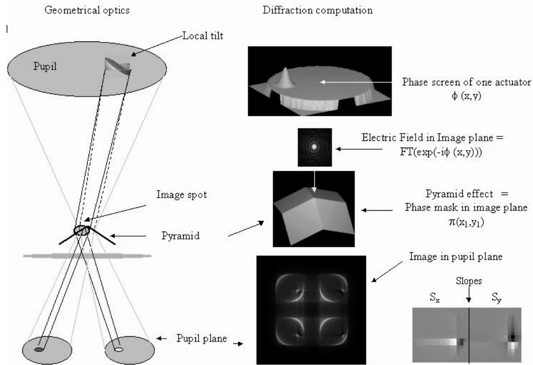
Figure 1 : Simulation of the pyramid sensor. Left : concept in geometrical optics (for a prism). Right : model based on Fraunhofer diffraction theory used in the simulations.
