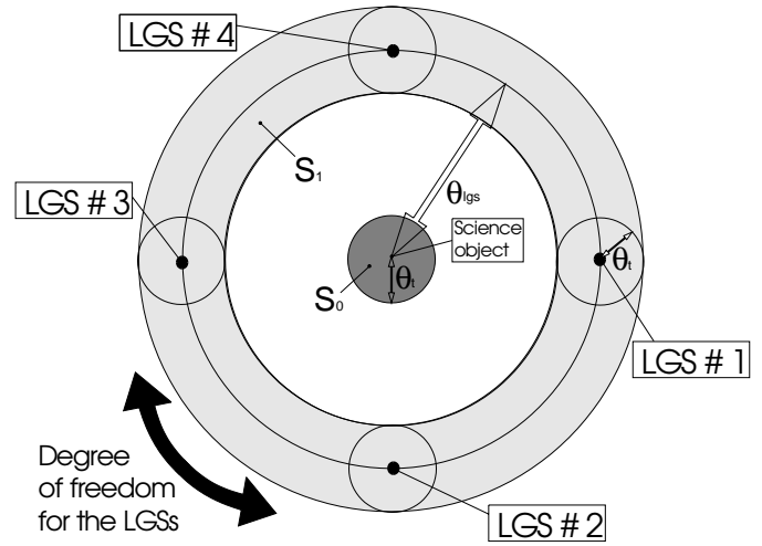
Fig. 1. Schematics of the geometry of the problem, with the various notations used in the text. S_2 is the whole area inside the outermost circle.
